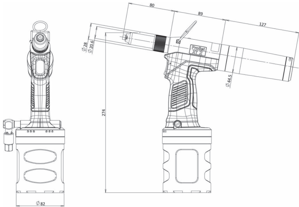
Dimensionen in Millimeter.
